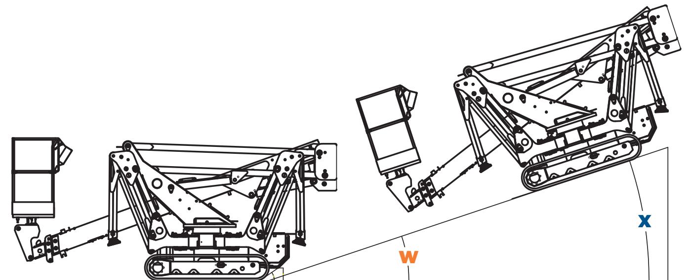
Maximum Slope Approach Angle 57%
