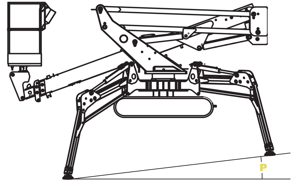
Maximum Slope to Stabilize 36%
